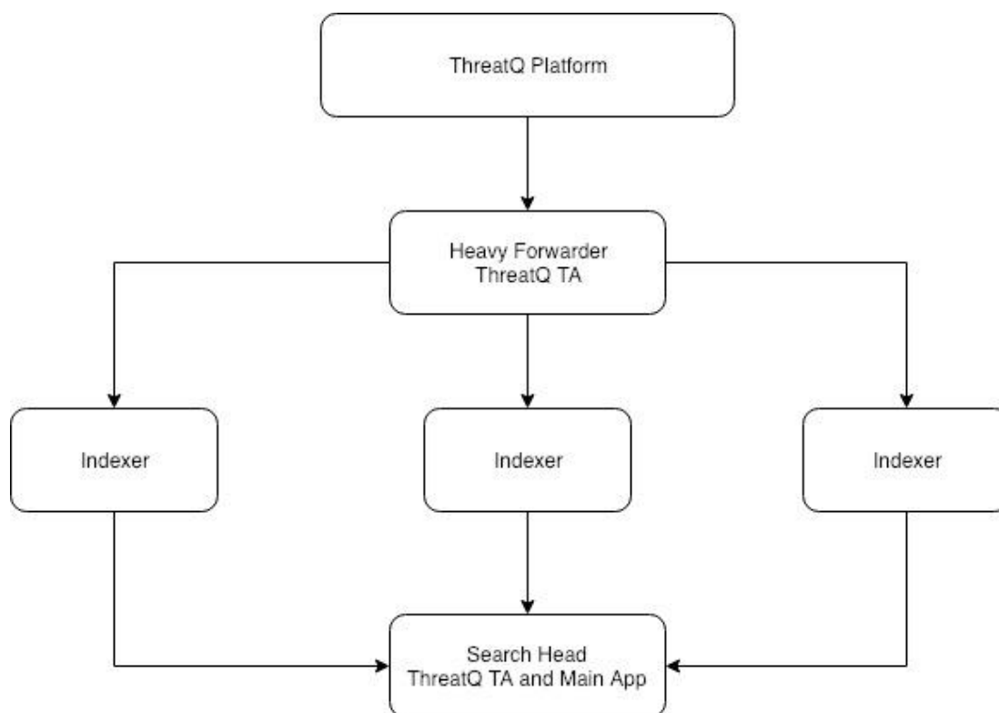
Figure 2: Deployment of Splunk App in Distributed Environment
